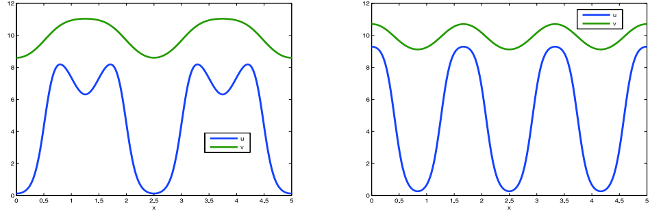
Figure 5: unstable solution 2teeth (left) and stable solution 2,3peak (right)
