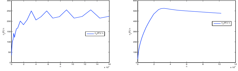
Figure 2: \frac{n_z(R')}{n} for SMD (left) and RCM (right) ordering in case 1
