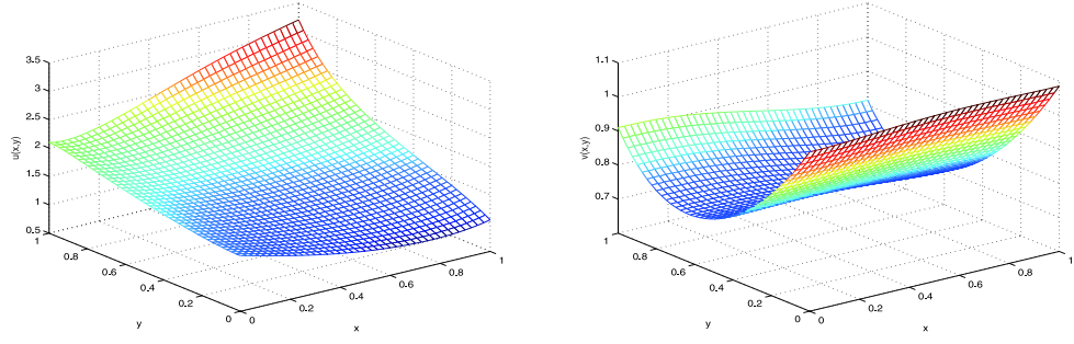
Figure 8: Solutions u (left) and v (right) for problem (4.4) in Case II
