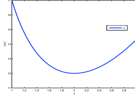
Figure 4: solution u for problem (4.1)
