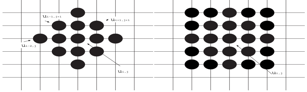
Figure 1: u_{k,l} involved in some constraint with u_{i,j} in case 1 (left) and case 2 (right)
