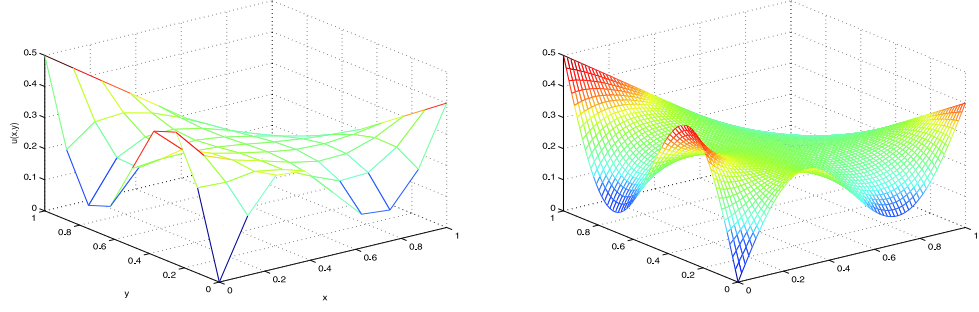
Figure 7: Stable solution u for problem (4.4) in Case I
