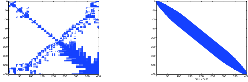
Figure 3: R' obtained by SMD (left) and RCM (right) orderings in case 1 with n = 400
