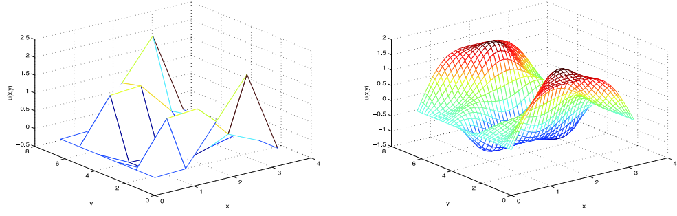
Figure 10: Solution for nonlinear wave equation (4.9), objective F_1
