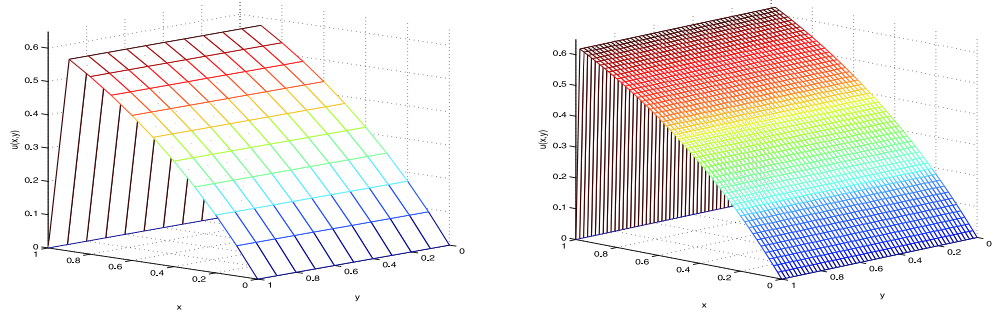
Figure 14: Solution u for problem (4.13)
