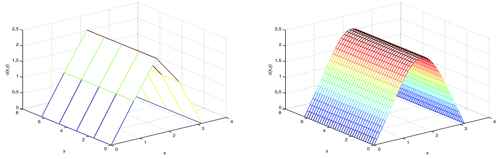
Figure 11: Solution for nonlinear wave equation (4.9), objective F_2
