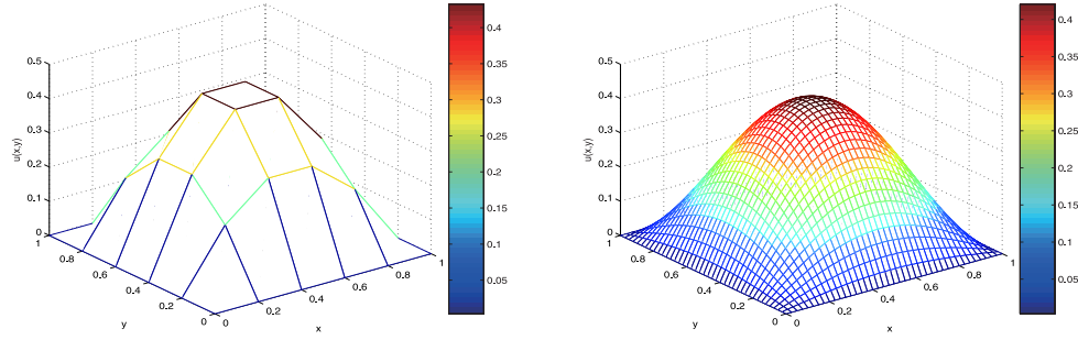
Figure 9: Solution for (4.5) if \lambda = 22 , (N_x, N_y) = (6, 6) and (N_x, N_y) = (41, 41)
