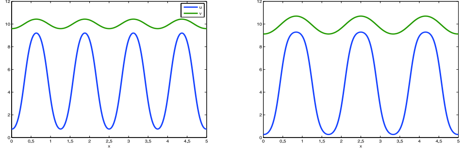
Figure 6: Stable solutions for grid-refining strategy 3a/b
