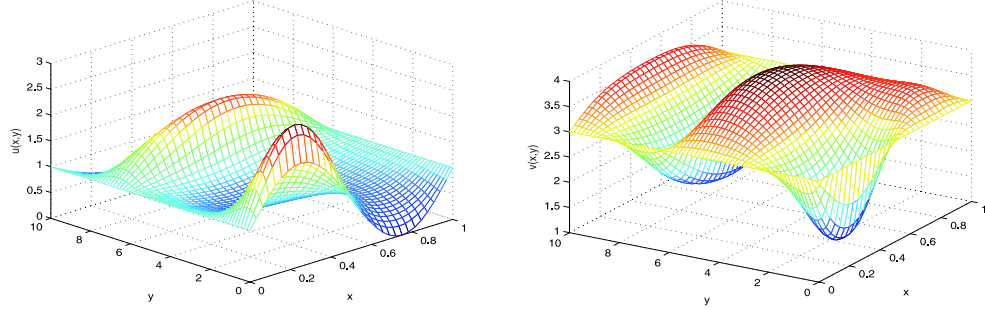
Figure 13: Solutions u (left) and v (right) for diffusion problem (4.11)
