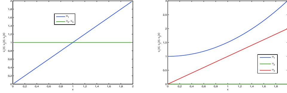
Figure 15: Solutions u^2 (left) and u^1 (right) of DAE problem (4.14)
